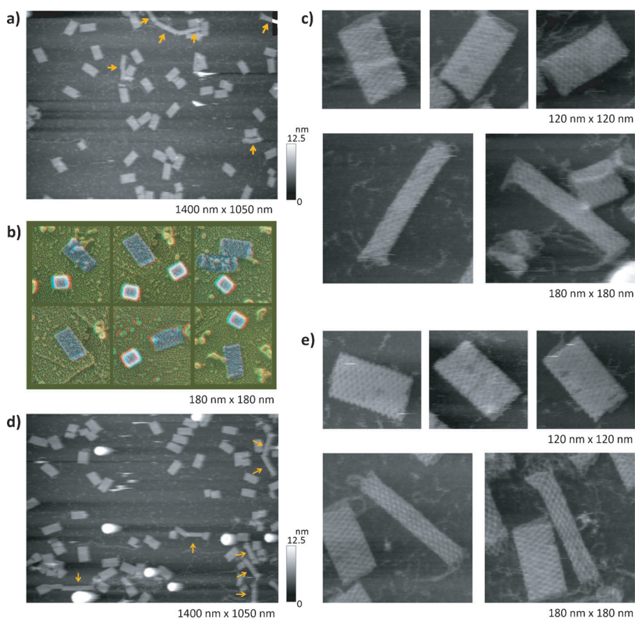
Figure 2. AFM images of helical tubes and their detailed surface patterns. a) AFM image of the 8-tubes after assembly. The orange arrows represent long tubular structures. b) Electron microscope images of short 8-tubes obtained using the quick-freeze/mica flake technique. The smaller cylinder in the images is hemocyanin (right-handed helical structure). c) Detailed AFM images of individual short and long 8-tubes. d) AFM image of the 8'-tubes after assembly. The orange arrows represent long tubular structures. e) Detailed AFM images of individual short and long 8'-tubes.
